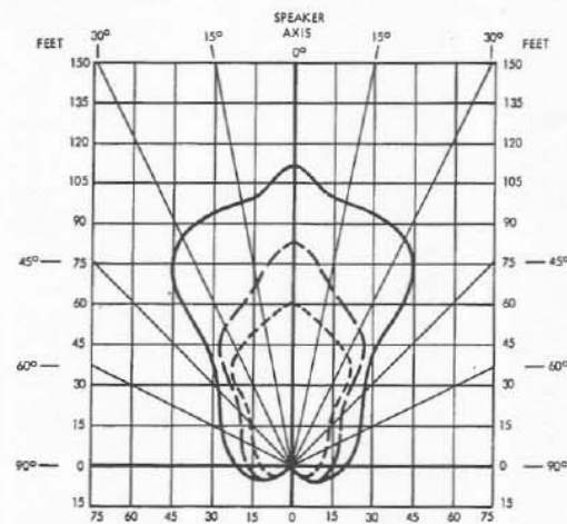
Figure 6-Constant Loudness Contour
