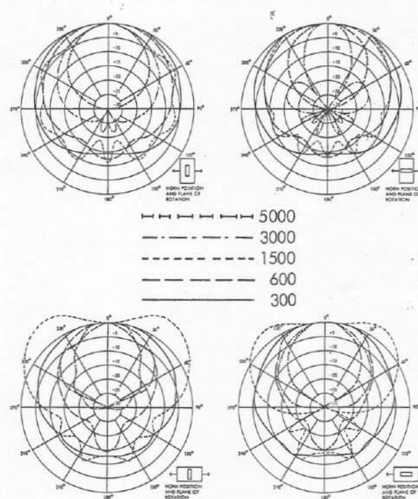
Figure 7-Polar Patterns
