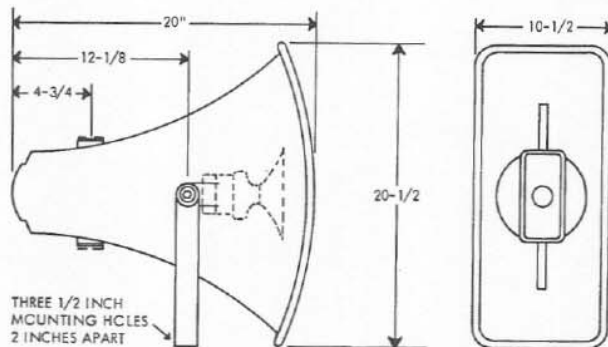
Figure 1 - Dimensions
